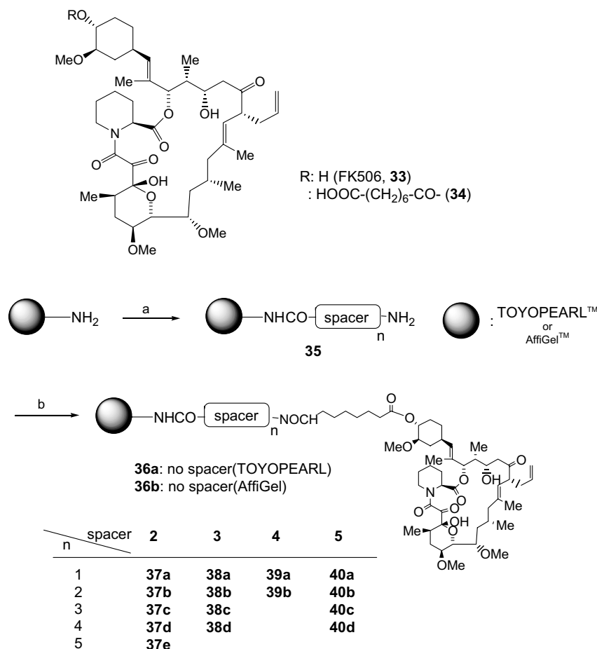
Scheme 3. Synthesis of affinity matrices bearing a FK506 derivative ( 34 ) with/without hydrophilic spacers ( 36–40 ): Reagents and conditions: (a) (i) N -Fmoc protected novel hydrophilic spacer ( 20 , 27 , 29 , or 32 ), PyBOP, DIPEA/NMP; (ii) piperidine/DMF/CH 2 Cl 2 = 1:2:2; (b) 34 , EDC·HCl, HOBt/DMF.
