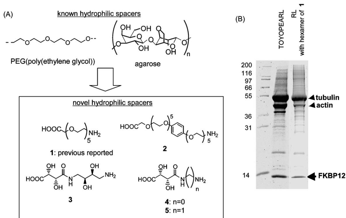
Figure 1. (A) Design of hydrophilic spacers studied in this study. (B) Binding proteins on TOYOPEARL bearing FK506 with and without previous reported hydrophilic spacer 1 . FKBP12 is known as the target protein of FK506, and other proteins such as tubulin and actin are thought to be nonspecific binding proteins.
