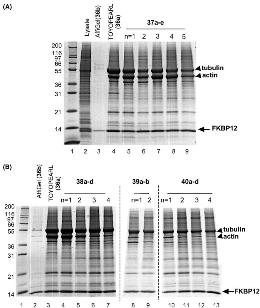
Figure 2. Binding proteins on affinity matrices bearing FK506 with or without hydrophilic spacers (36–40).
