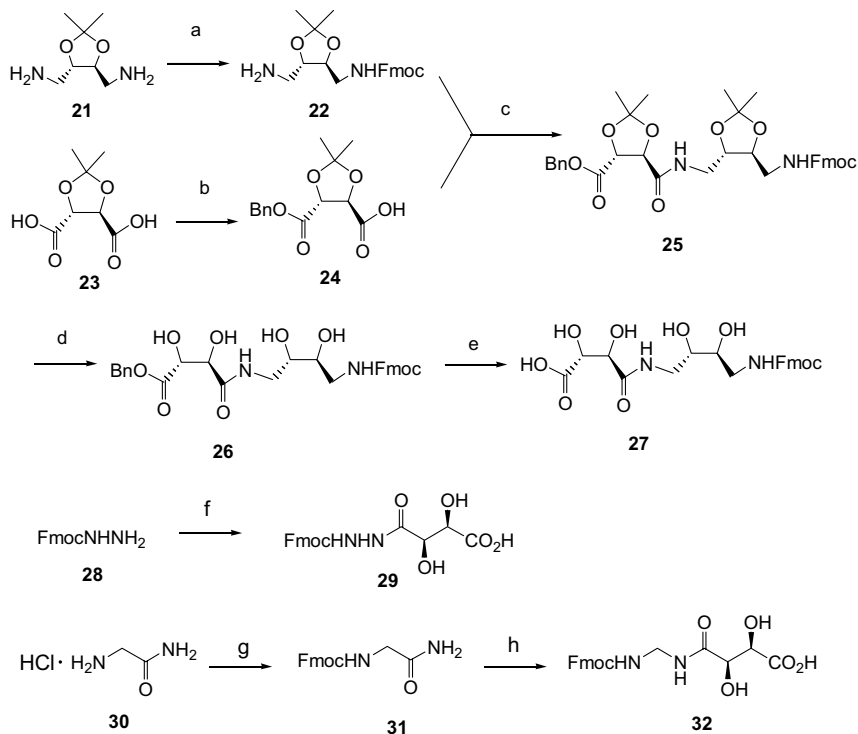
Scheme 2. Synthesis of N -Fmoc protected 3 ( 27 ), 4 ( 29 ), and 5 ( 32 ): Reagents and conditions: (a) Fmoc-OSu, NEt 3 /THF; (b) BnOH, CDI, DBU/CH 3 CN; (c) PyBOP, DIPEA/DMF; (d) 80% TFA/CH 2 Cl 2 ; (e) H 2 , Pd(OH) 2 /MeOH, AcOEt; (f) L-(+)-tartaric acid, EDC·HCl/DMF; (g) Fmoc-OSu, Na 2 CO 3 /acetone, water; (h) (i) PhI(OCOCF 3 ) 2 /AcOEt-CH 3 CN-H 2 O, (ii) L-(+)-tartaric acid, EDC·HCl/DMF.
