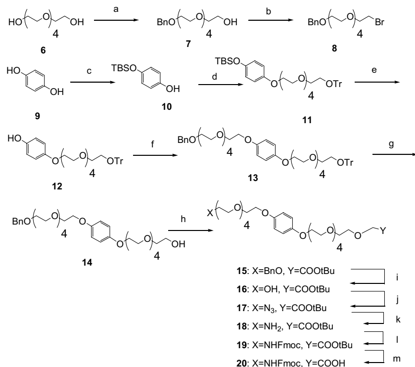
Scheme 1. Synthesis of N -Fmoc protected 2 ( 20 ): Reagents and conditions: (a) BnCl, KOH; (b) PPh 3 , CBr 4 /CH 2 Cl 2 ; (c) TBSCl, imidazole/DMF; (d) TrO(CH 2 CH 2 O) 5 H, PBu 3 , DAMD/toluene; (e) TBAF/THF; (f) 8 , NaH/THF; (g) TFA/CH 2 Cl 2 , H 2 O; (h) BrCH 2 COO t Bu, NaH/THF, DMF; (i) H 2 , Pd(OH) 2 /MeOH; (j) (i) TsCl, DMAP/Py, (ii) NaN 3 /DMF, (k) H 2 , Pd(OH) 2 /MeOH; (l) Fmoc-OSu, NEt 3 /THF; (m) 95% TFA/H 2 O.
