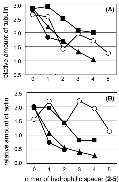
Figure 3. Plots of estimated amount of tubulin and actin with numbers of hydrophilic spacer 2 (○), 3 (■), 4 (●), and 5 (▲). The amounts of tubulin and actin were represented as a ratio compared to amount of FKBP12.
